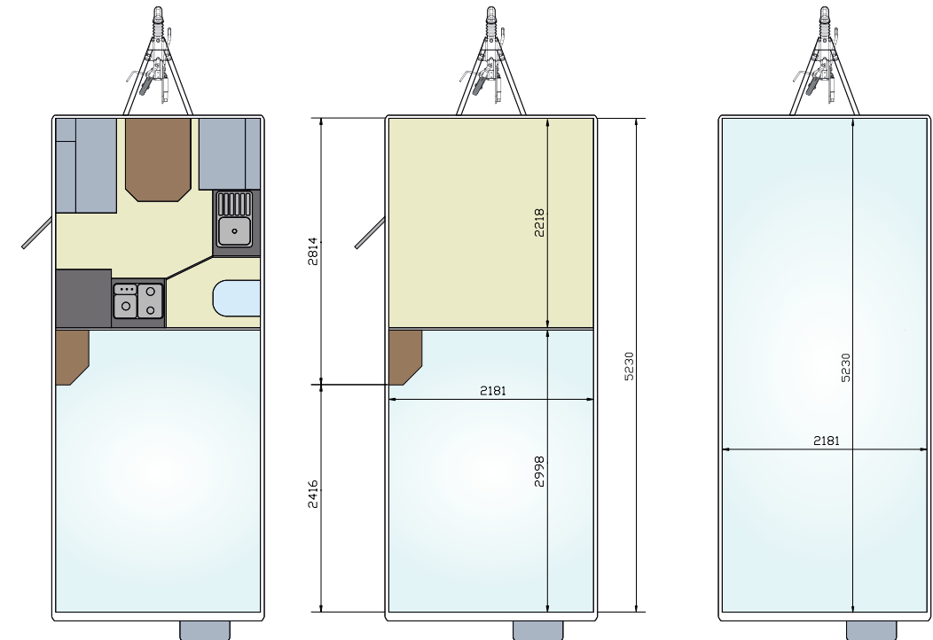
Trailer showing living accommodation layout
