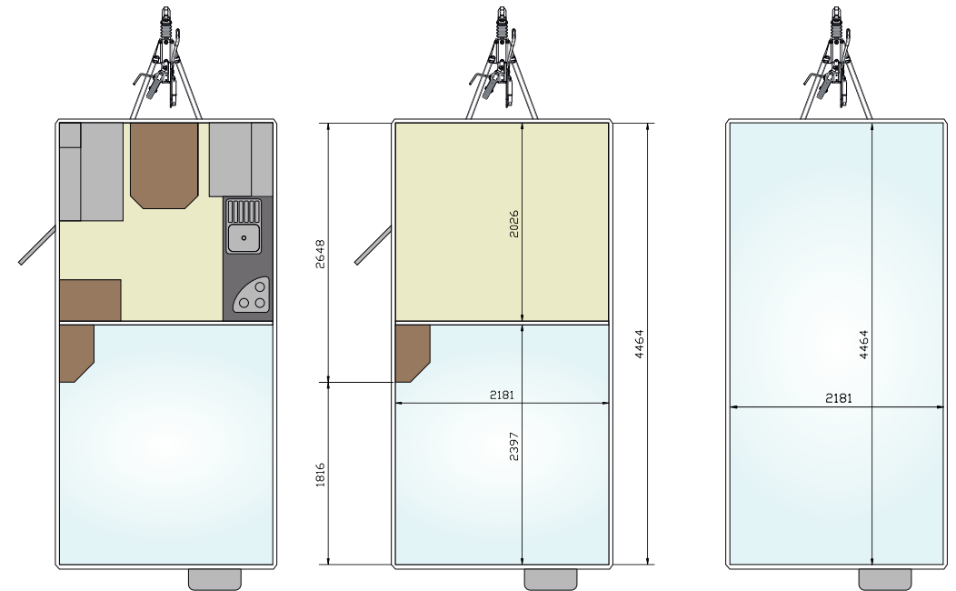
Trailer showing living accommodation layout
